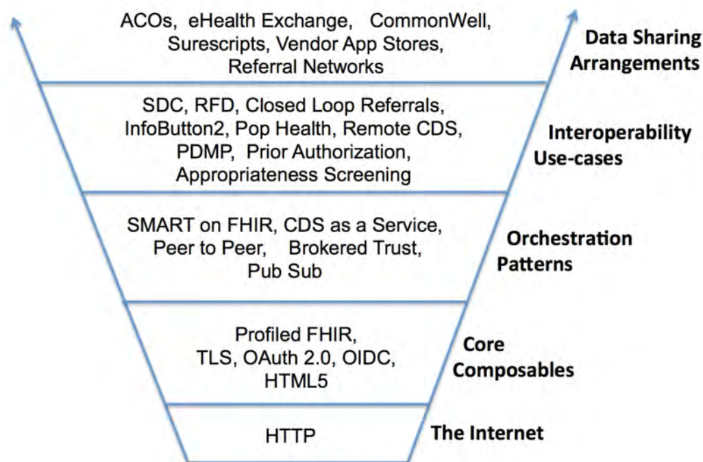
Figure 4: Example Health IT Hourglass Instantiation
